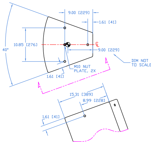
M10 EYE BOLT ANGLE POINT, 12X
