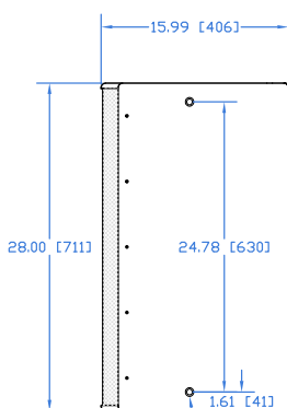
M10 EYE BOLT ANGLE POINT, 12X
