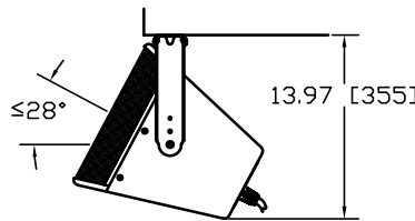
Tilt limited to point where enclosure touches bracket
