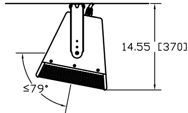
May be tilted >79^\circ with optional barrier strip input
