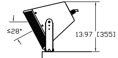
Tilt limited to point where enclosure touches bracket
