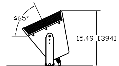
May be tilted >65^\circ with optional barrier strip input
