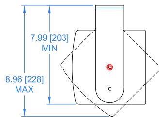
MOUNTING POSITION 1
