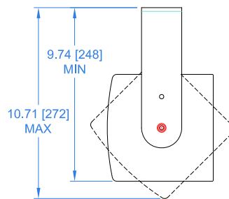
MOUNTING POSITION 2
